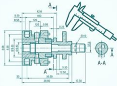
Tool drawings
